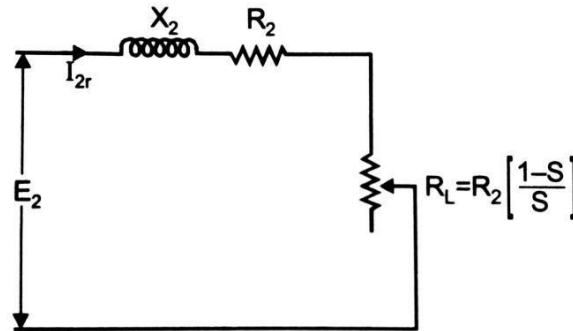
Fig.4.9. Equivalent circuit of rotor
