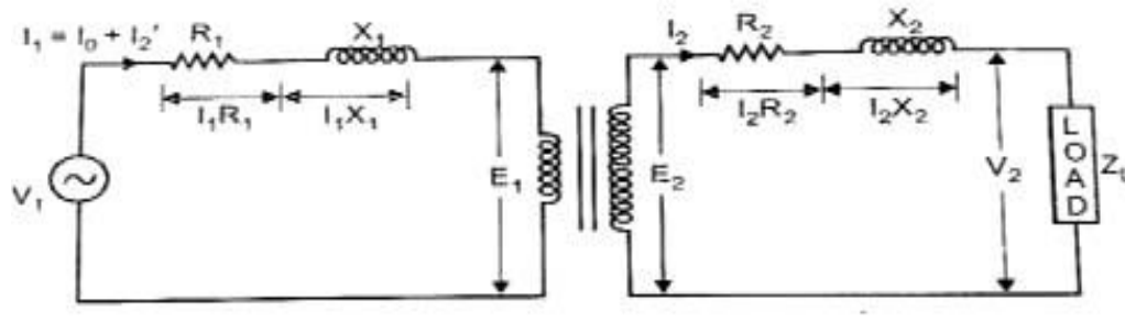
Fig 2.18: Transformer with resistances and leakage reactance
