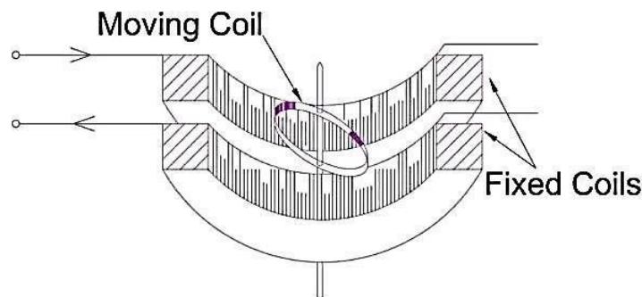
Fig 4.9 Electrodynamicometer wattmeter
