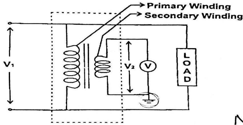
Fig. 4.22 Potential Transformer
