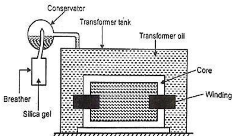
Fig 2.4: Transformer construction
