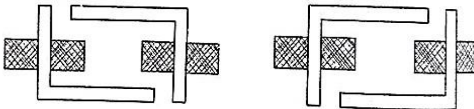
Fig 2.2: L- type stampings
