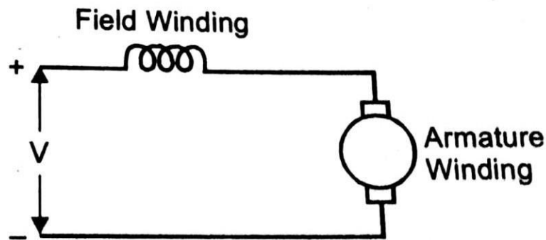
Fig 3.26 universal motor
