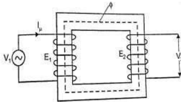
Fig 2.9: Ideal transformer
