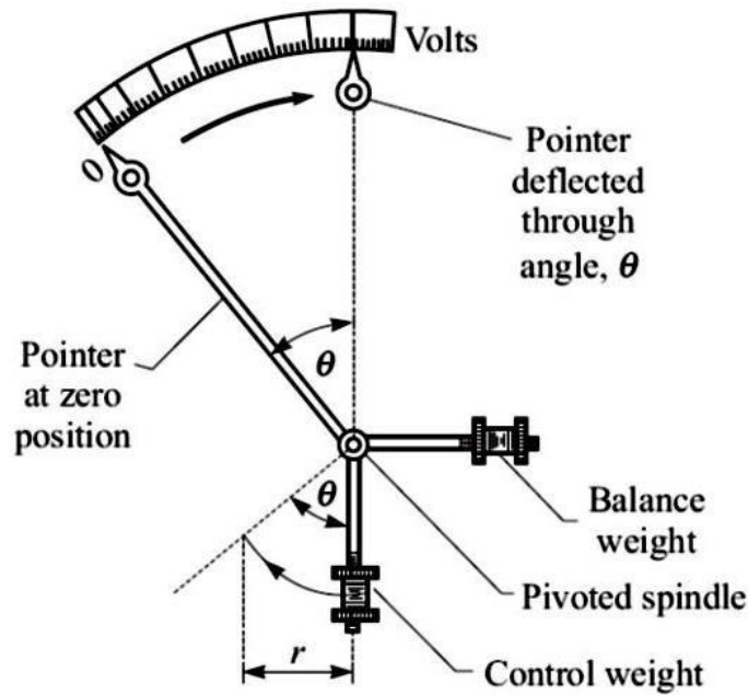
Figure 4.5: Gravity control
