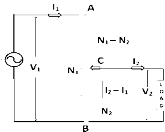
Fig 2.25 Auto transformer design
