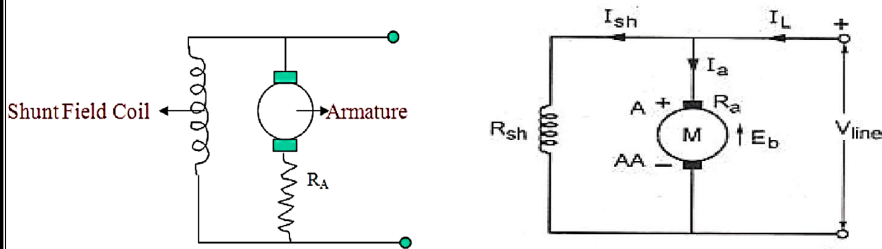
Fig 3.19: Connection of a shunt motor
