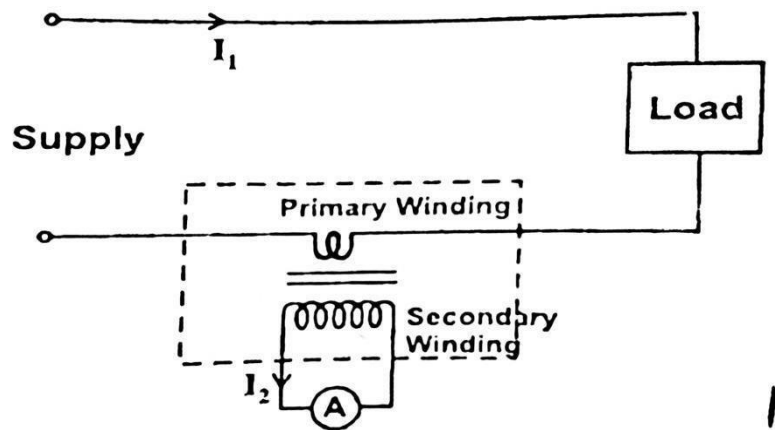
Fig. 4.21 Current Transformer
