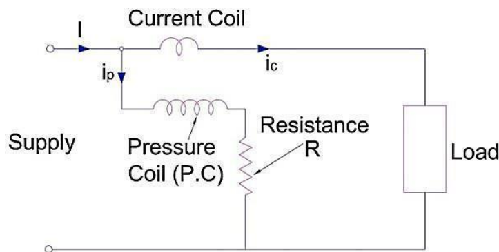
Fig 4.10 electric circuit of electrodynamic wattmeter
