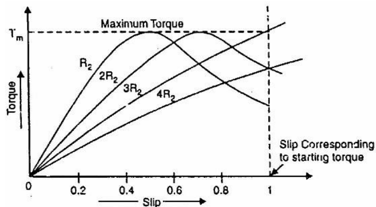
Figure 4.13 Torque-Slip characteristics
