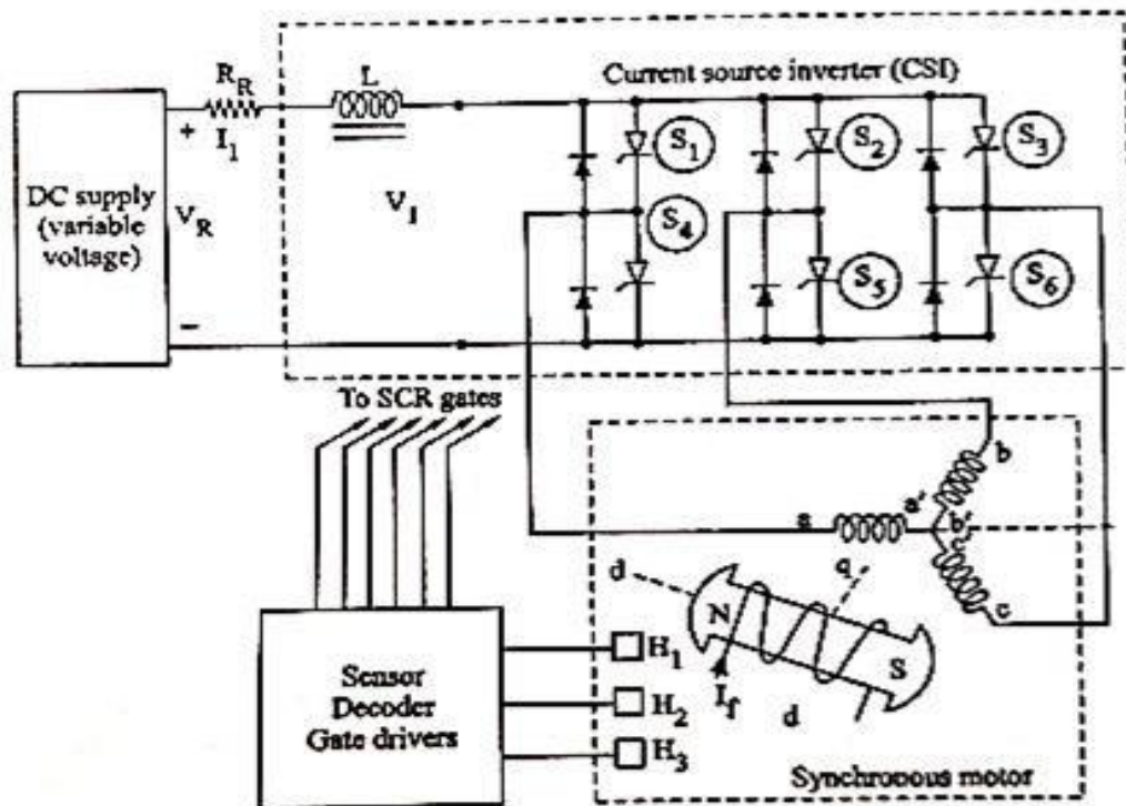
Fig 4.48: Brushless DC motor
