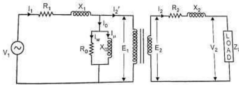
Fig 2.19: Transformer circuit
