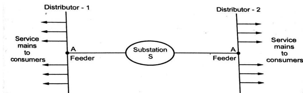
Figure 5.3: Radial distribution system
