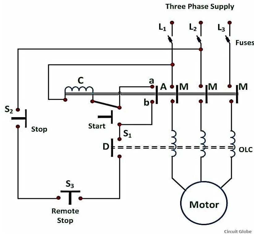
Fig 4.14 DOL starter
