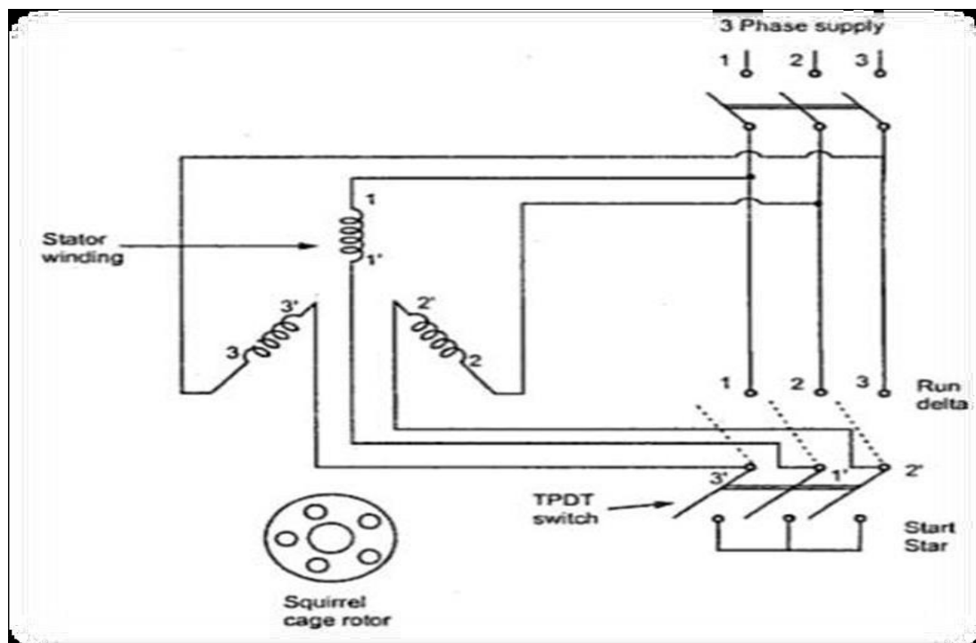
Figure 4.17 Star-delta starter
