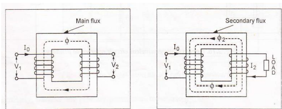
Fig 2.13: transformer under no-load and loaded condition
