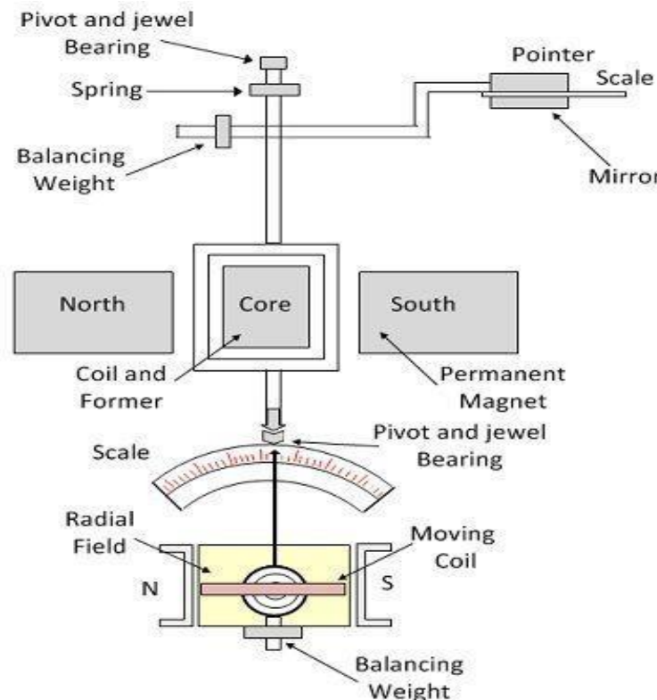
Figure 4.6: PMMC
