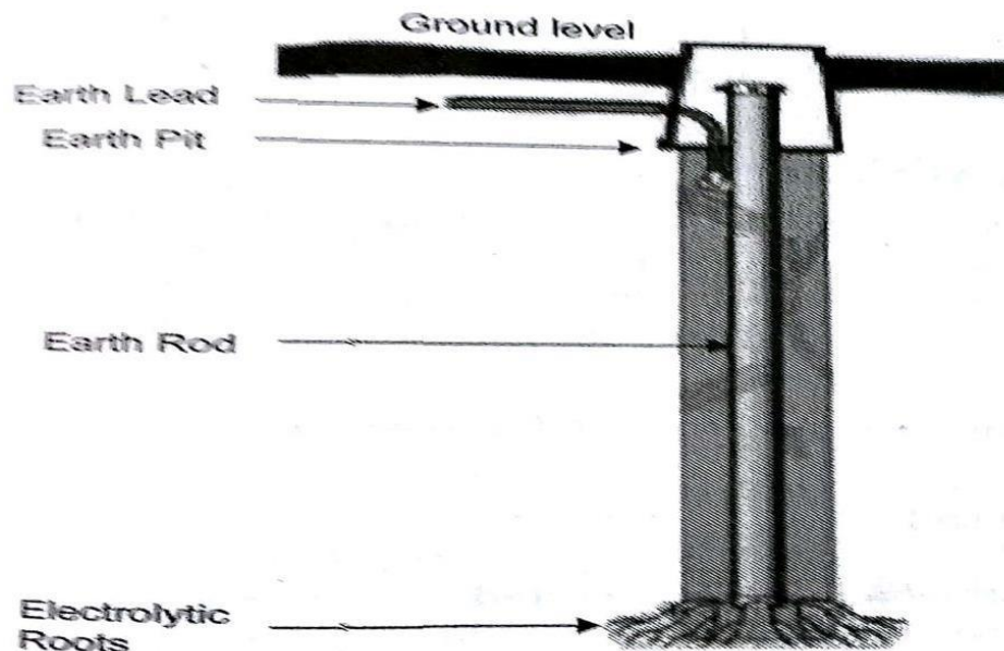
Figure 5.11: Rod Earthing
