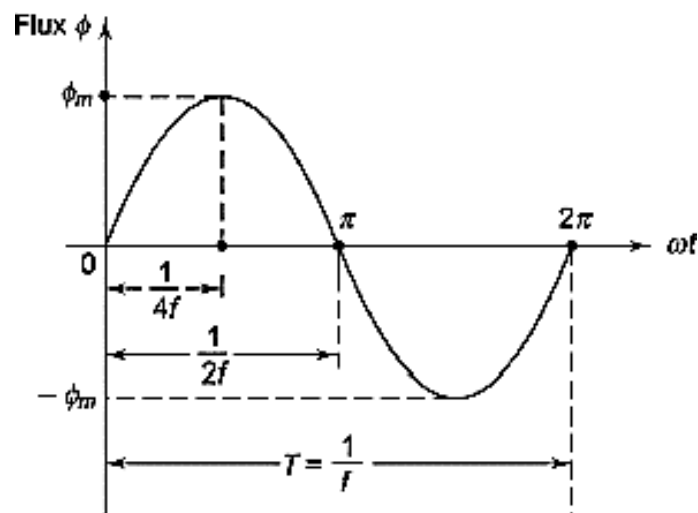
Fig 2.8: output waveform
