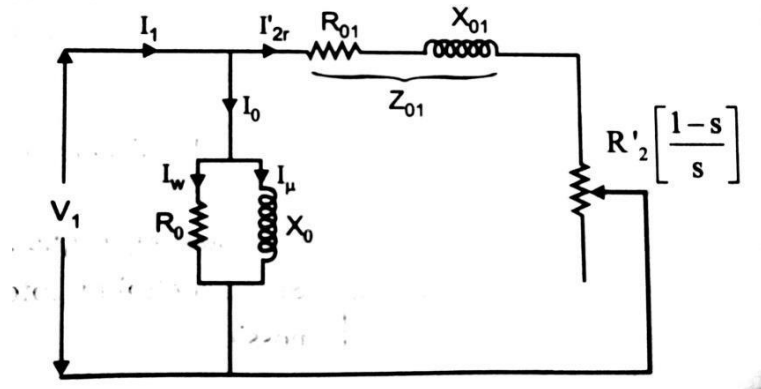
Fig.4.12 Approximate Equivalent circuit
