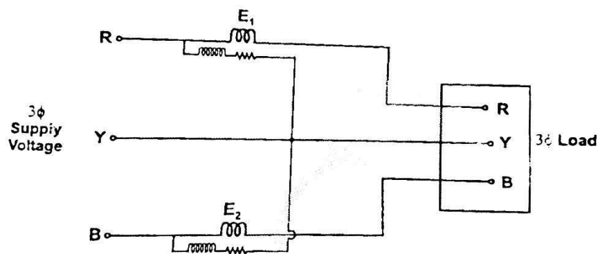
Fig. 4.17 Circuit diagram of 2 element energy meter
