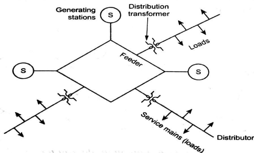
Figure 5.5: Interconnected system
