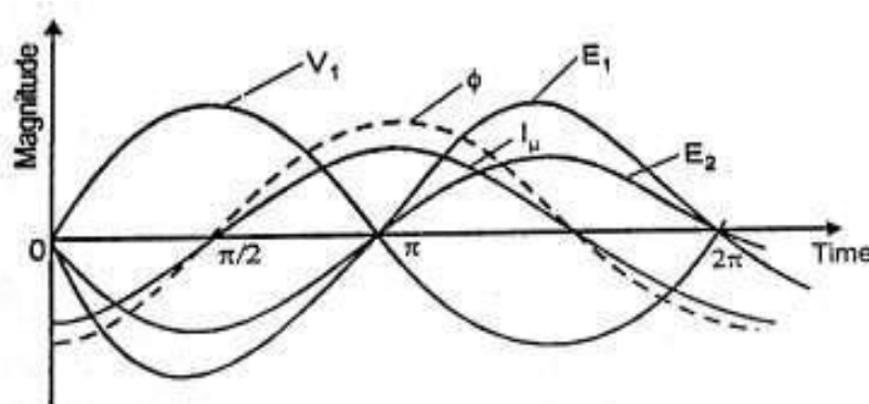
Fig 2.10: Output waveform
