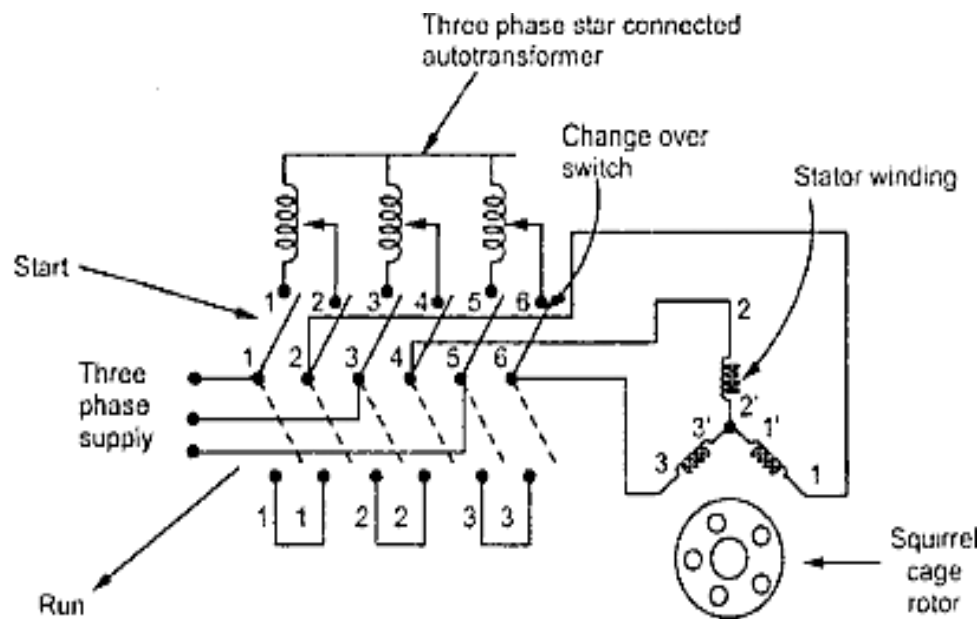
Figure 4.16 Autotransformer starter
