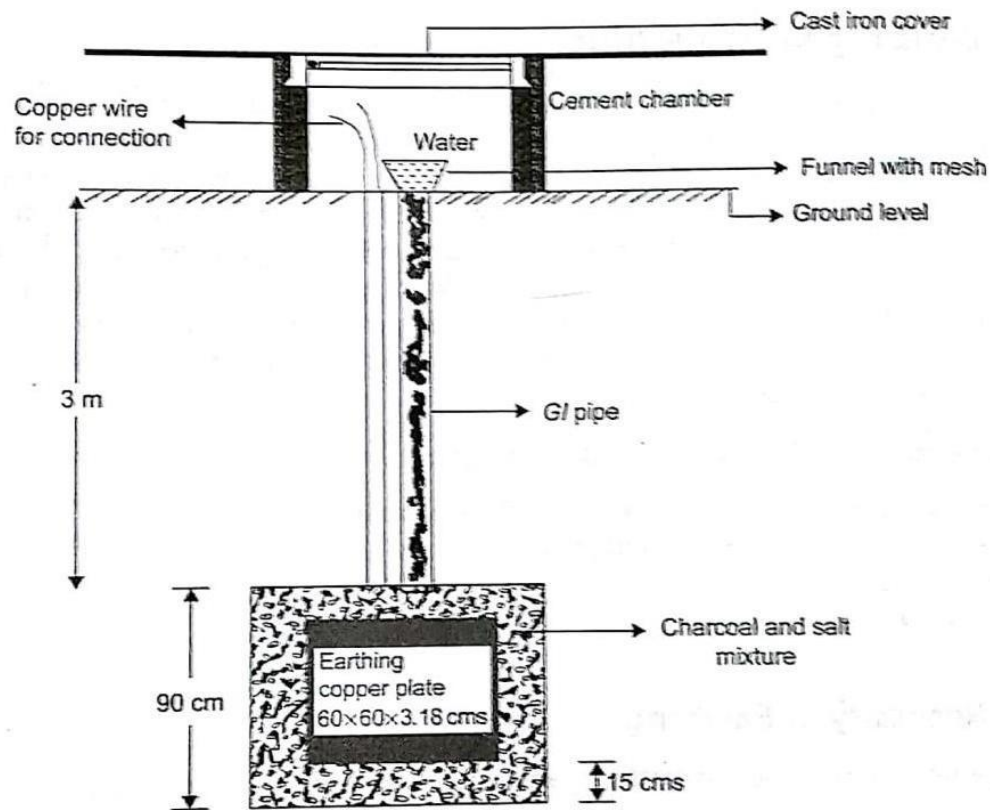
Figure 5.9: Plate Earthing
