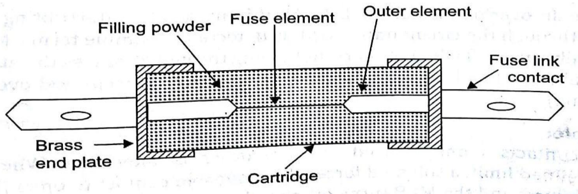
Figure 5.14: Cross section of HRC Cartridge Fuse
