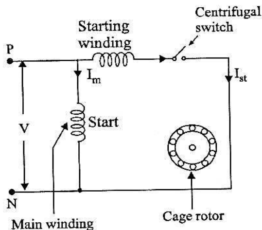
Fig 4.27 Split phase induction motor
