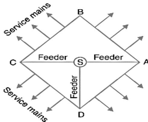
Figure 5.2: Distribution Systems
