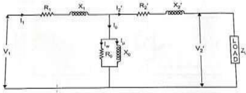
Fig 2.20: Equivalent circuit of a transformer referred to primary
