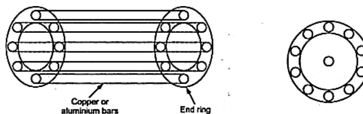
Figure. 4.18 Cage type rotor
