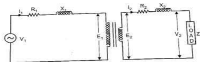
Fig 2.15: Practical transformer on load
